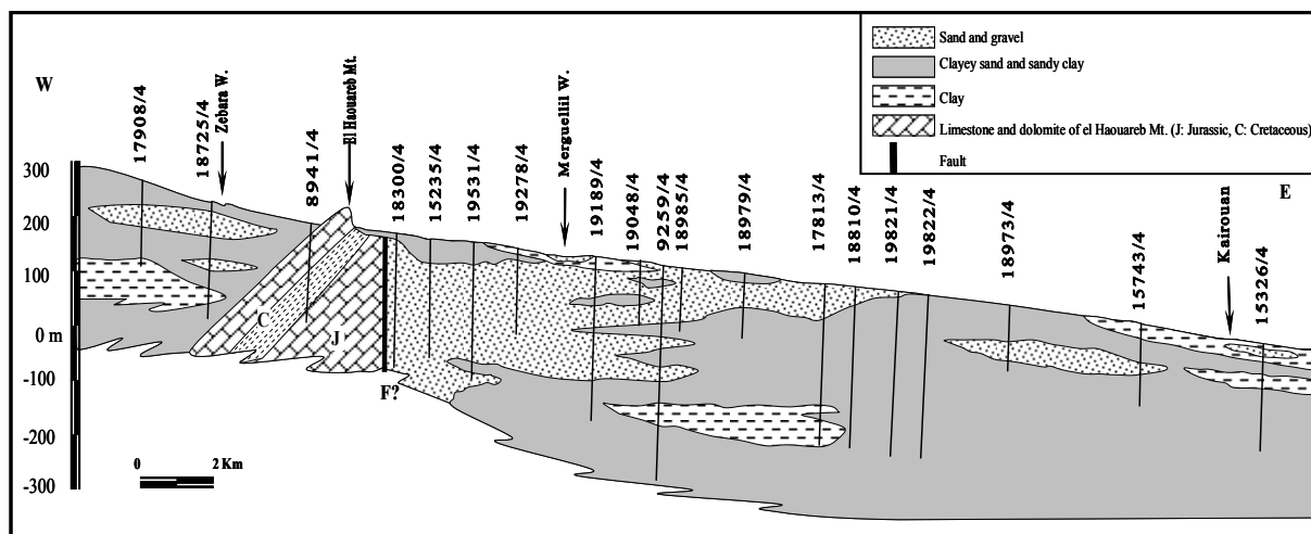
Fig. 2 W-E geological cross-section along Wadi Merguellil: the Tertiary and Quaternary Aïn el Beidha aquifer to the west; the Mesozoic karst of Jebel el Haouareb; the thick Quaternary aquifer of the Kairouan plain to the east (whole thickness not represented).
